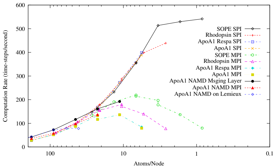
Fig. 1: This figure compares the strong scaling characteristics of the Blue Matter MPI and BG/L ADE SPI-based implementations for the molecular systems described in Table 1. The simulation parameters employed for the SOPE and Rhodopsin systems were those used in production, specifically a Verlet integrator with P3ME being computed on every time-step. For ApoA1, we attempted to match the parameters used by the NAMD benchmark as closely as possible, but we were forced to use a larger, 128 \times 128 \times 128 , mesh for our FFT because our current implementation is restricted to dimensions that are powers of two. This plot also includes data reported for NAMD on Blue Gene/L [14] and for the Lemieux Alpha system at the Pittsburgh Supercomputing Center [13]. Because benchmarking data for NAMD was not available for the SOPE and Rhodopsin system, the only comparison possible was on the 92,224 atom ApoA1 system. The NAMD benchmarks used a smaller FFT mesh size ( 108 \times 108 \times 80 ) than that used by Blue Matter ( 128^3 ) and on the Lemieux system used a specially tuned version of the Charm++ library written to the Elan communication library provided by Quadrics. On Blue Gene/L, NAMD results are shown for both a specially tuned version of the Charm++ library using a custom messaging layer and for an MPI-based implementation of Charm++[14].
